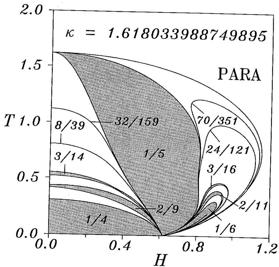
Fig. 17 T - H phase diagram for \kappa = 1.61803\dots , corresponding to q_c = 2\pi/5 .
