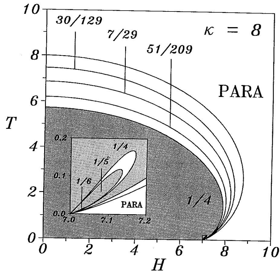
Fig. 18 T - H phase diagram for \kappa = 8 . The insert shows the detail near the multiphase point.
