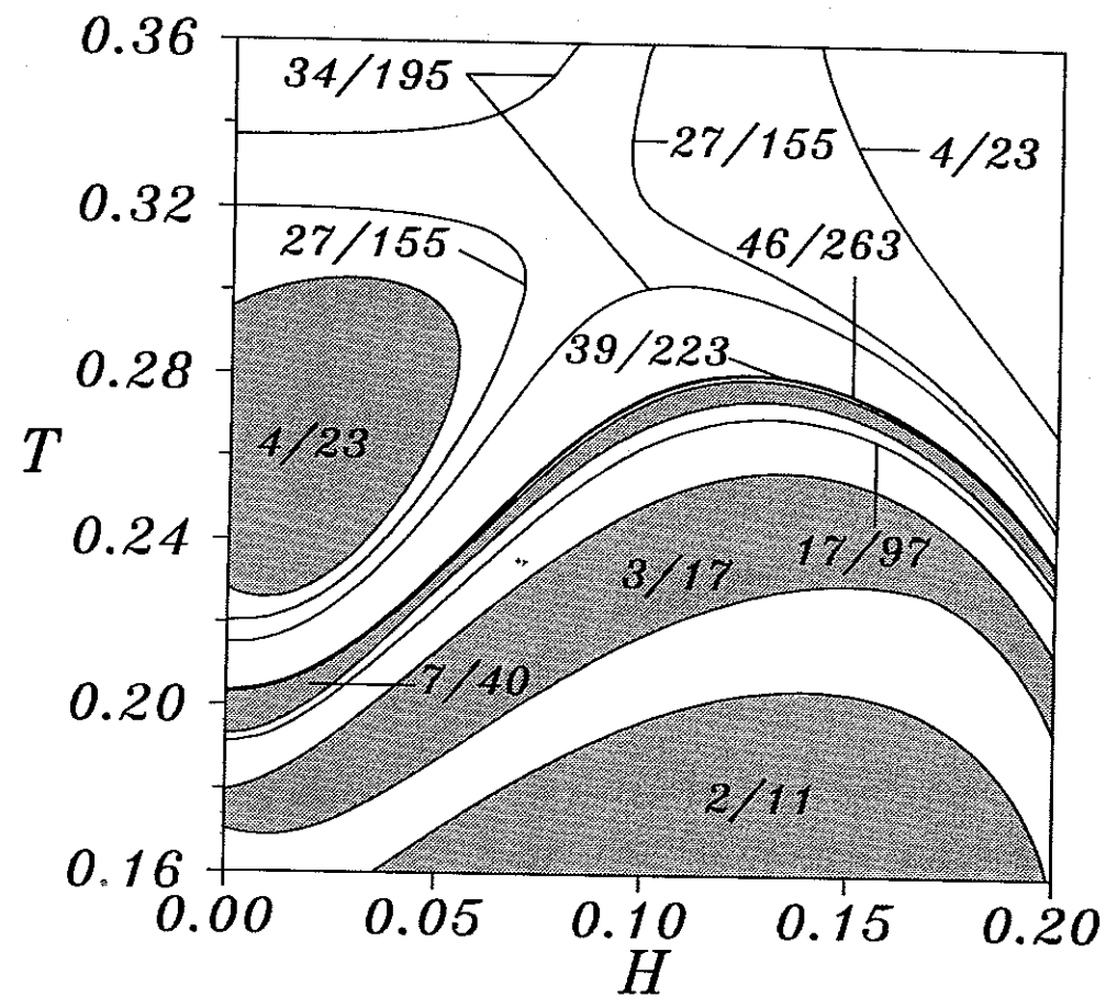
Fig. 14 Detail of the T - H phase diagram for \kappa = 1.1 .
