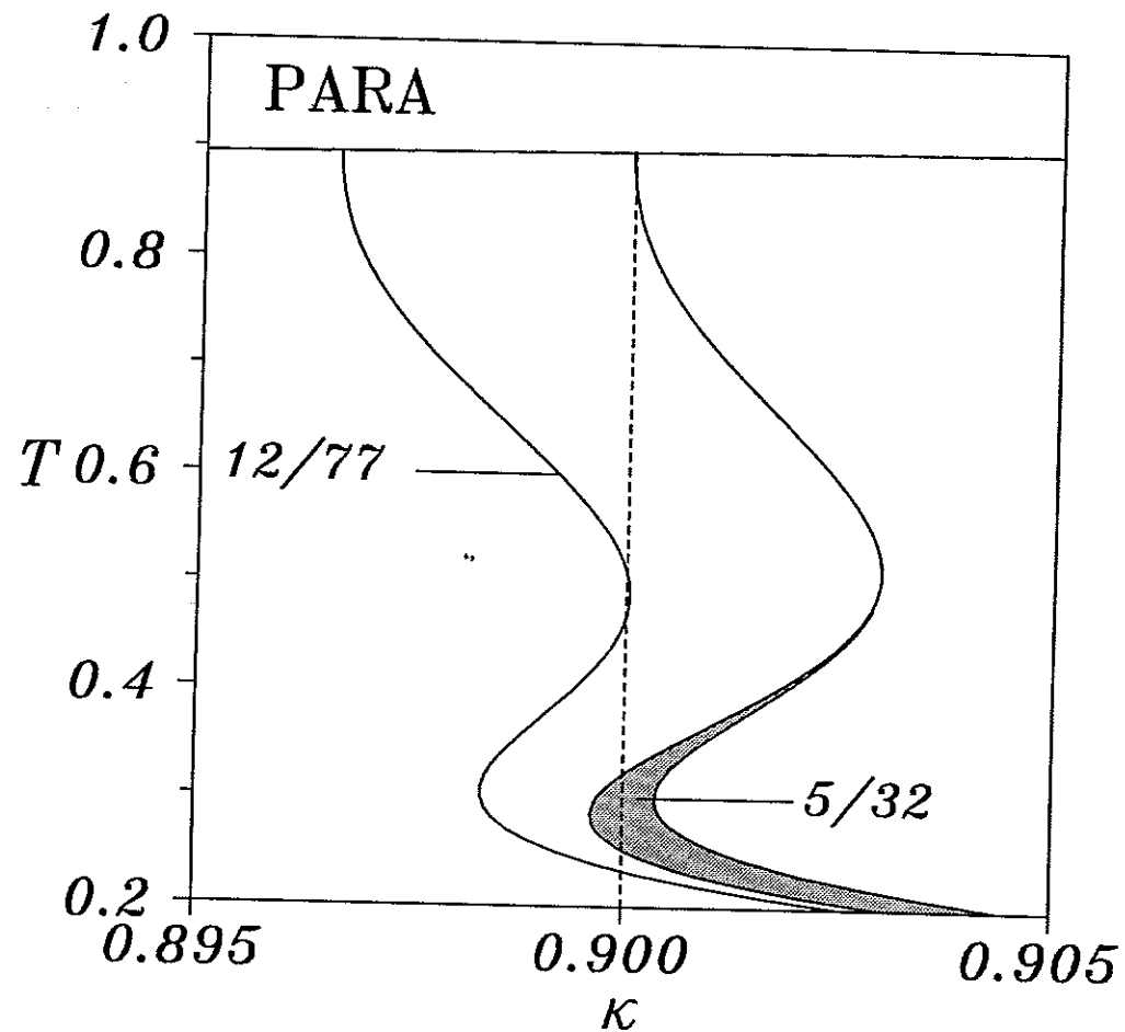
Fig. 10 Detail of the T - \kappa phase diagram in the neighborhood of \kappa = 0.9 . The phases 5/32 and 12/77 recur two and three times, respectively, as the temperature is lowered for \kappa = 0.9 .
