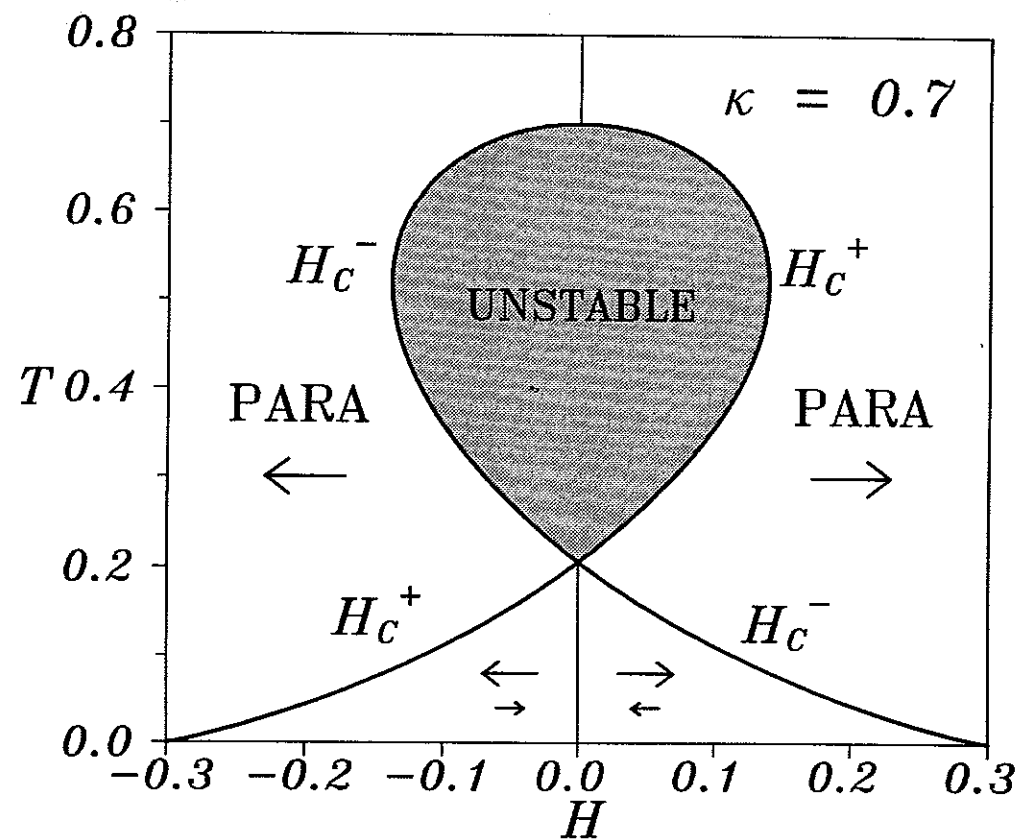
Fig. 4 Stability region of the paramagnetic phase for \kappa = 0.7 . Inside the tent shaped region there is a coexistence of two phases, with magnetizations parallel and antiparallel to the field, as indicated by the arrows. Inside the shaded bubble shaped region the paramagnetic phase is unstable.
