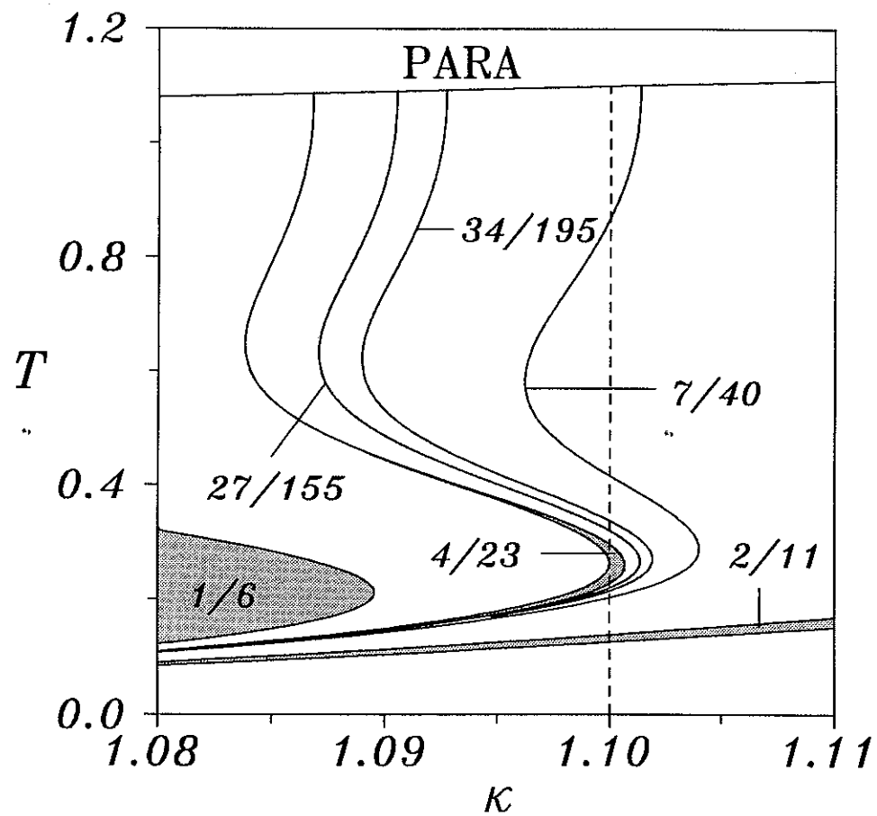
Fig. 15 Detail of the T-\kappa phase diagram in the neighborhood of \kappa = 1.1 . The phases 7/40 recurs three times as the temperature is lowered for \kappa = 1.1 .
