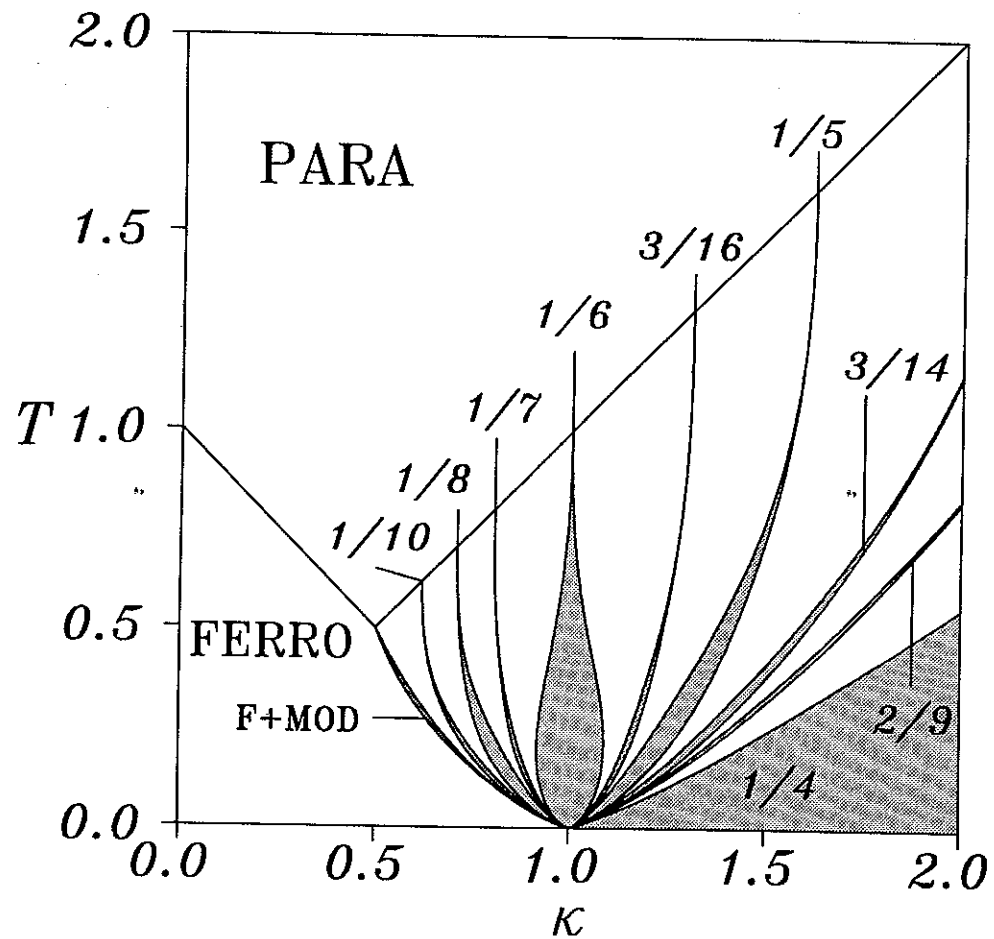
Fig. 7 Zero field T - \kappa phase diagram. Only the main commensurate phases (shaded regions) are indicated. In shaded region indicated by F+MOD the ferromagnetic and modulated phases coexist.
