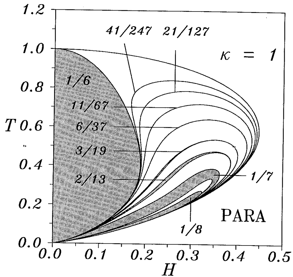
Fig. 11 T - H phase diagram for \kappa = 1 .
