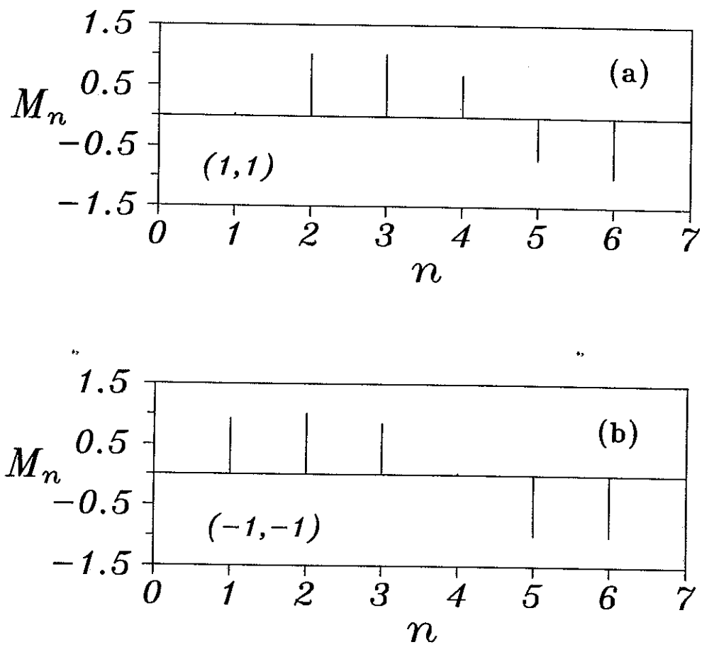
Fig. 19 Two distinct commensurate 1/6 structures that coexist for \kappa = 1.08 , T = 0.2 and H = 0.24 . They can be obtained by iterating the map with the initial conditions (a) (1, 1) and (b) (-1, -1) .
