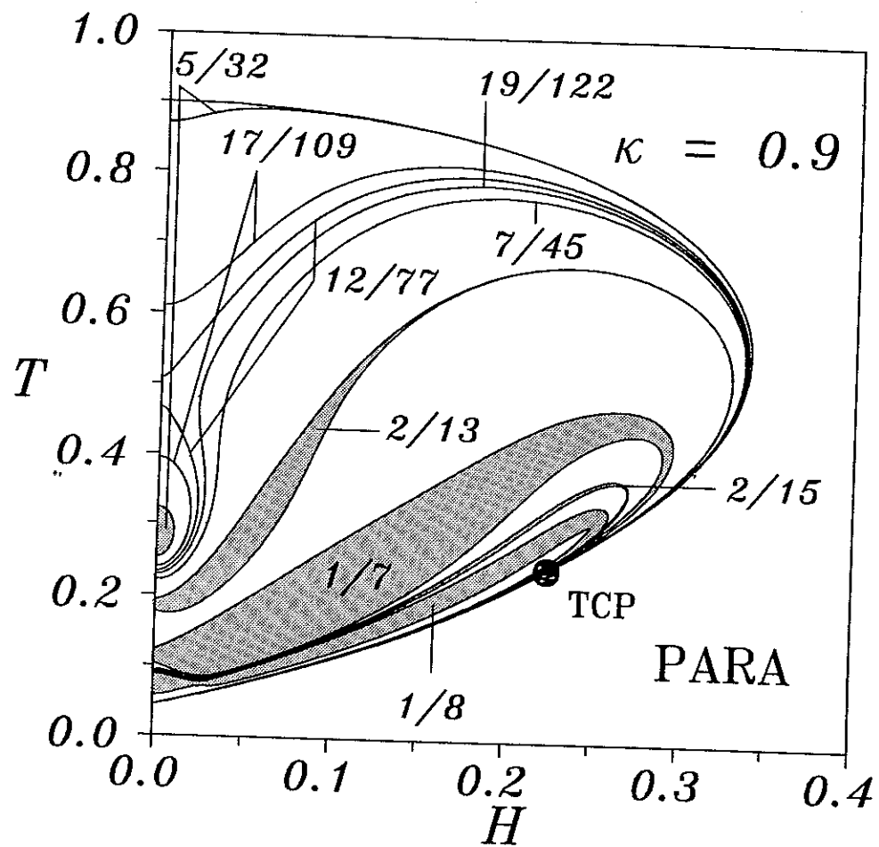
Fig. 9 T - H phase diagram for \kappa = 0.9 . Observe the existence of disjoint commensurate phases and the pinching of the 1/8 phase. The coexistence region between paramagnetic and modulated phases is too narrow to be visible at the scale of the figure, and ends at the tricritical point (TCP).
