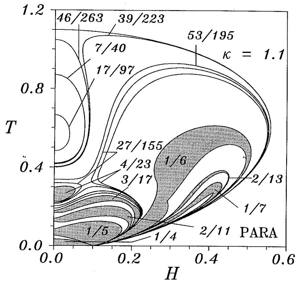
Fig. 13 T - H phase diagram for \kappa = 1.1 .
