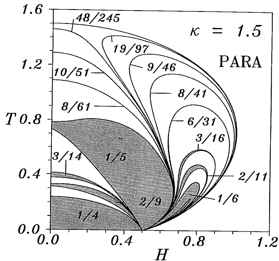
Fig. 16 T-H phase diagram for \kappa = 1.5 .
