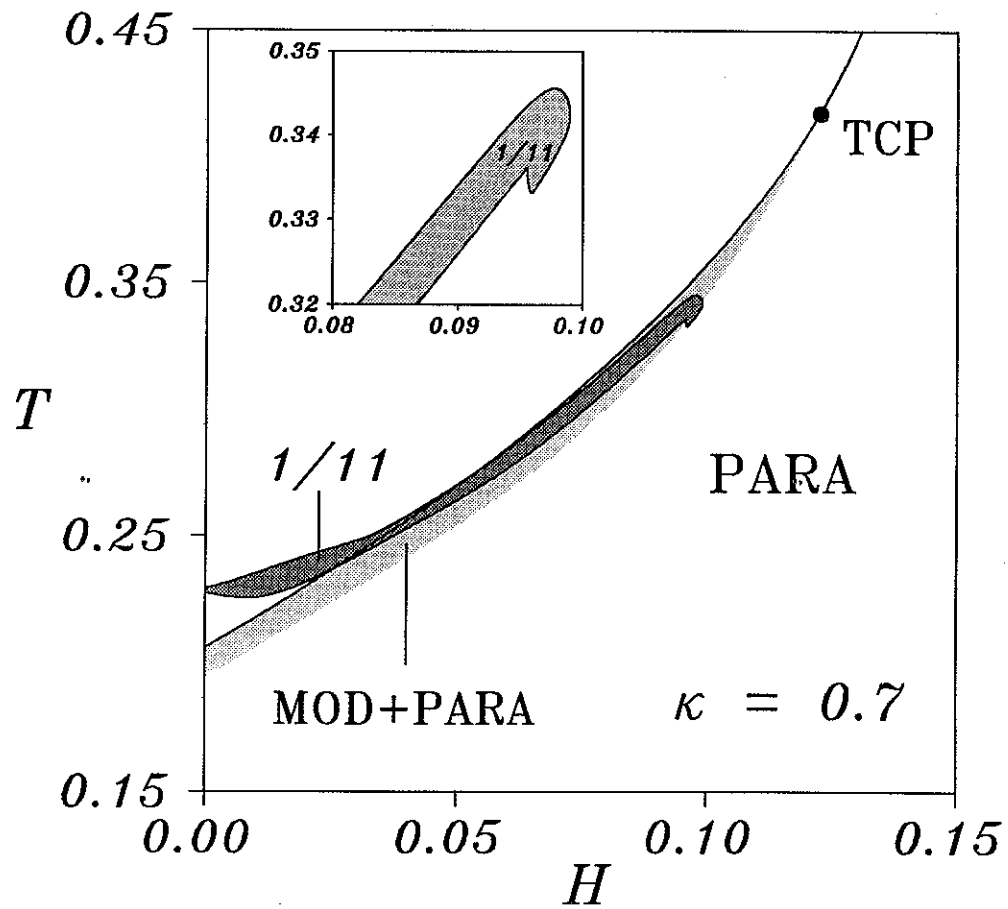
Fig. 25 The 1/11 phase for \kappa = 0.7 (dark shaded). In light shaded region paramagnetic and modulated phases coexist.
