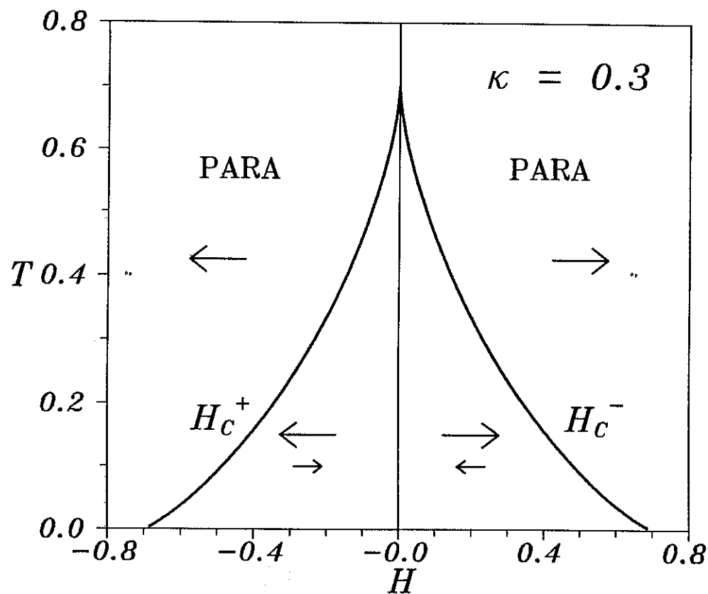
Fig. 3 Stability region of the paramagnetic phase for \kappa = 0.3 . Inside the tent shaped region there is a coexistence of two phases, with magnetizations parallel and antiparallel to the field, as indicated by the arrows.
