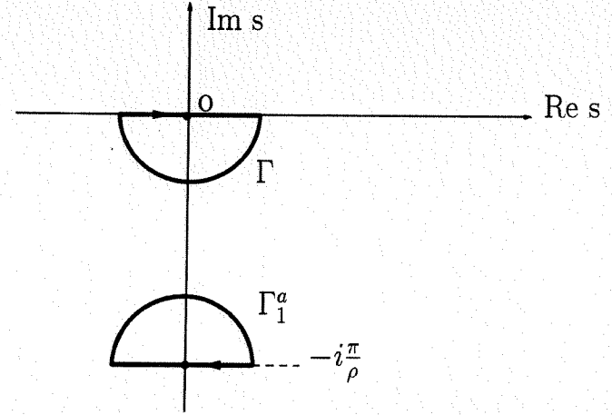
FIG. 2. Contours of integration \Gamma, \Gamma_1^a
