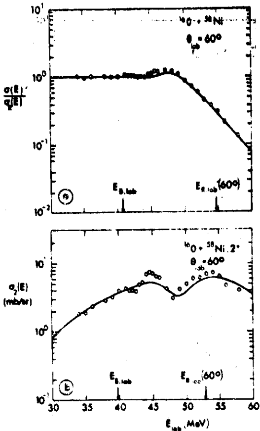
Fig. 8.1. Excitation functions \sigma(E) , \sigma_n(E) and \sigma_2(E) for elastic and inelastic scattering, respectively, of ^{16}\text{O} on ^{58}\text{Ni} at \theta_{lab} = 60^\circ . The curves are CF fits to the data of ref. [34] with parameters given in table 8.1.
