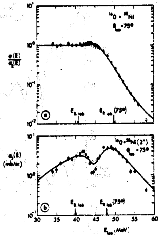
Fig. 8.2. Excitation functions \sigma(E) , \sigma_n(E) and \sigma_2(E) for elastic and inelastic scattering, respectively, on ^{16}\text{O} on ^{58}\text{Ni} at \theta_{lab} = 75^\circ . The curves are CF fits to the data of ref. [34] with parameters given in table 8.1.
